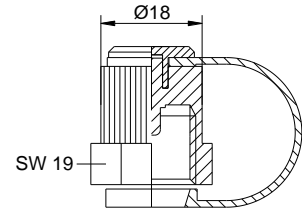
plastic cap (FAK) fig. 3
