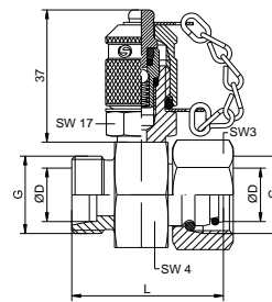
type DKOGE (DIN2353 / ISO8434-1 and -4)
